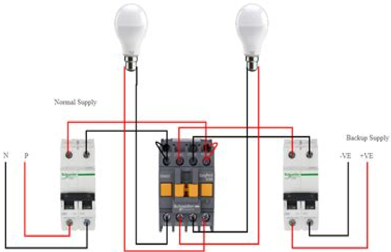
Automatic Changeover Switch Connection
