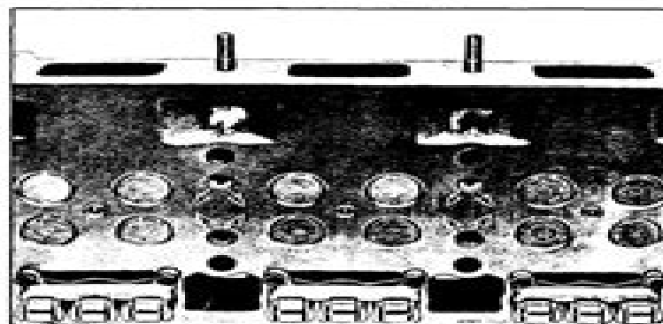
Fig. 5 - Correct Installation of Water Nozzles in Four-Valve Cylinder Head
