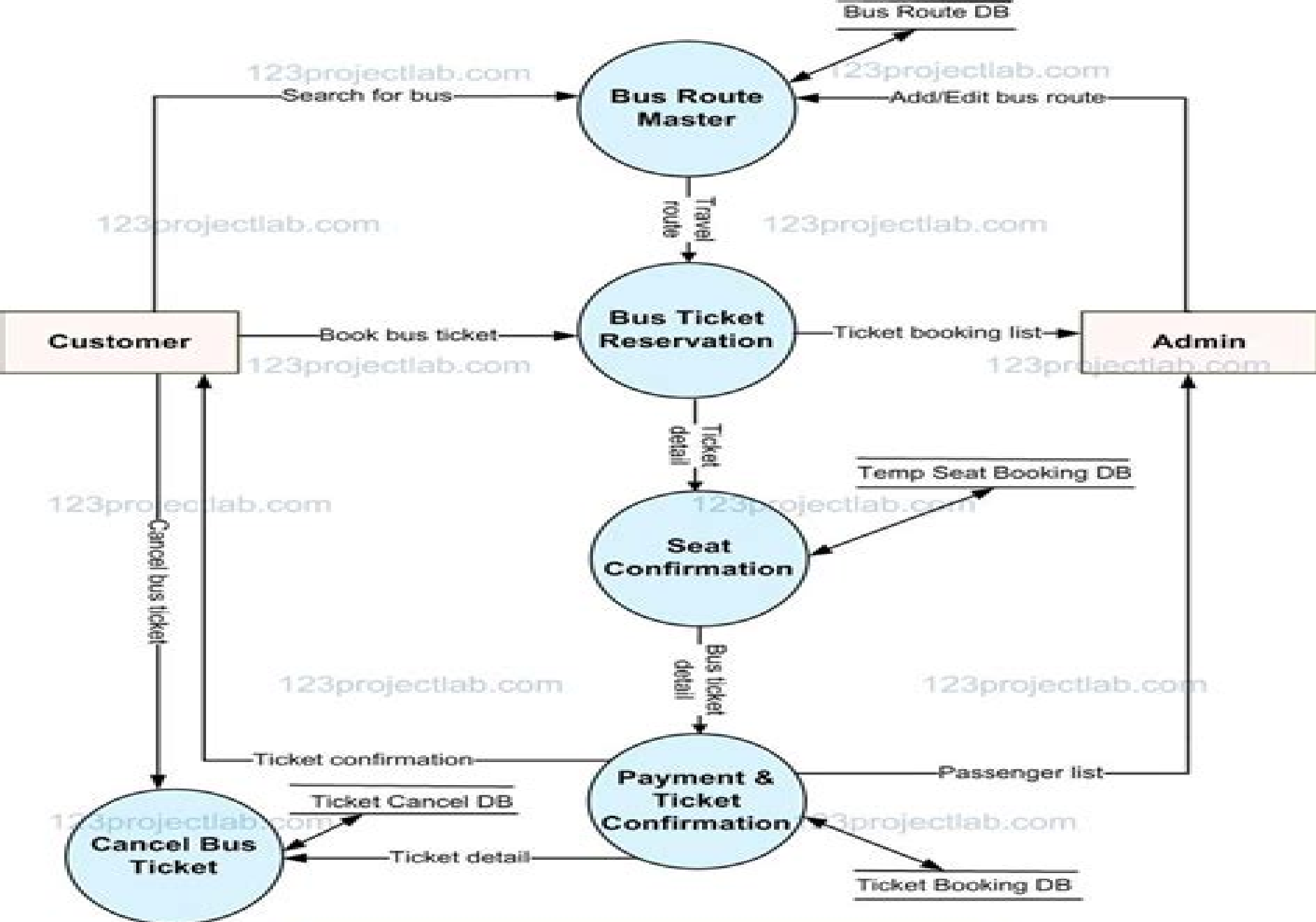
Level-2 DFD for Online Bus Ticket Booking System
