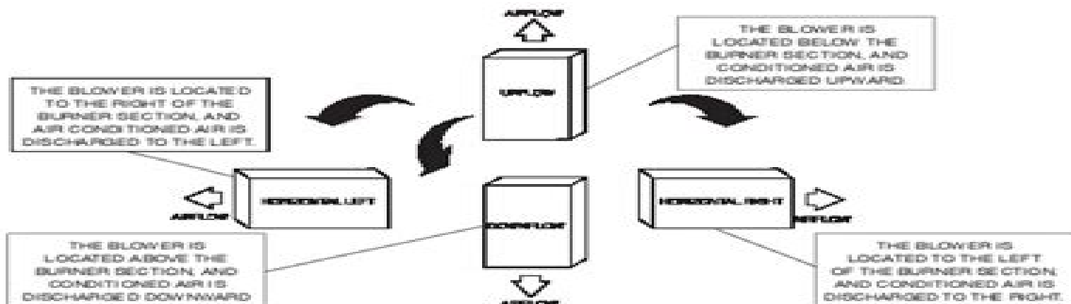
Fig. 4 - Multiple Orientations
