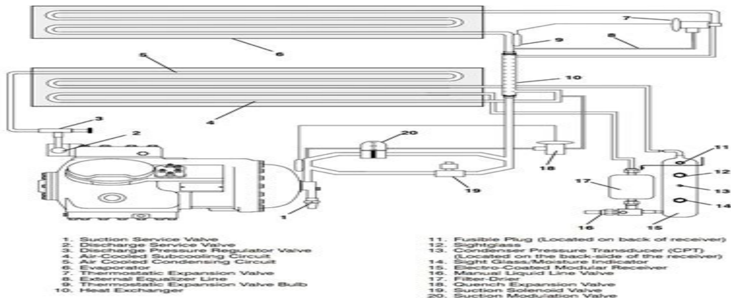
Figure 1-9. Refrigeration Circuit with Receiver and Subcooling Condenser Coil (Optional)
