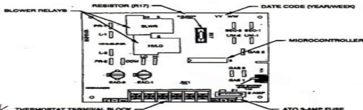
Fig. 3—Control Center Component Location
