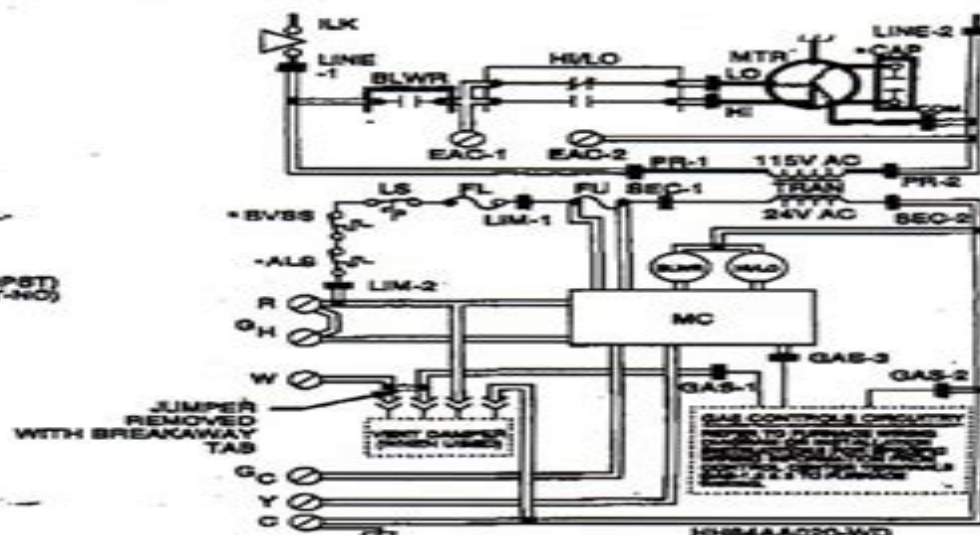
Fig. 2—Wiring Schematic
