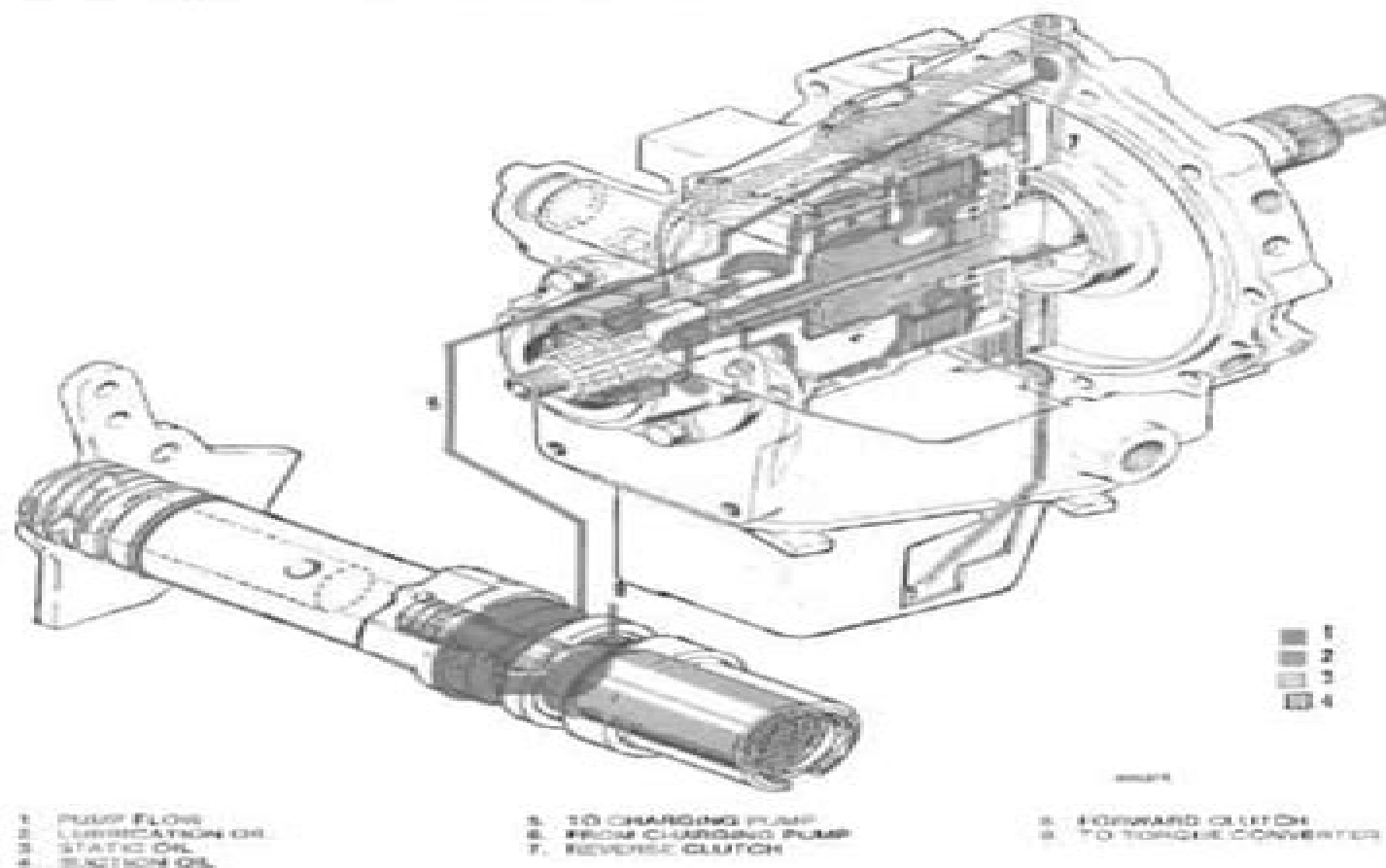
Figure 3 - Oil Flow in Neutral
