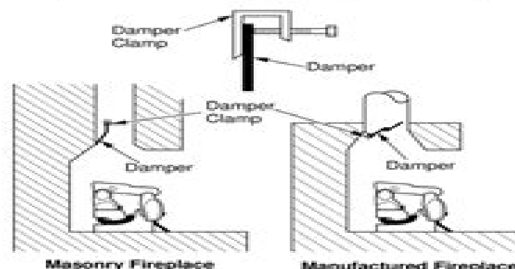
Figure 10 - Attaching Damper Clamp
