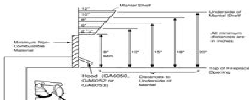
Figure 7 - Minimum Mantel Clearances When Using Hood
