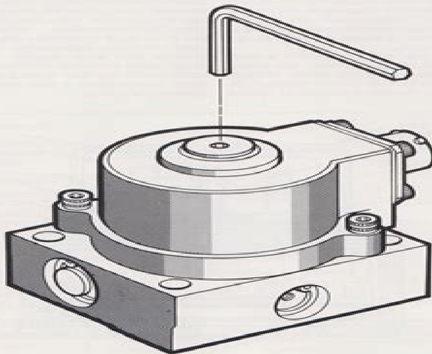
Fig 2 Optional mechanical null adjust
