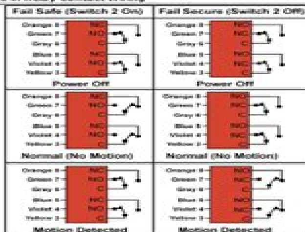
Figure 4: Relay Contact Wiring
