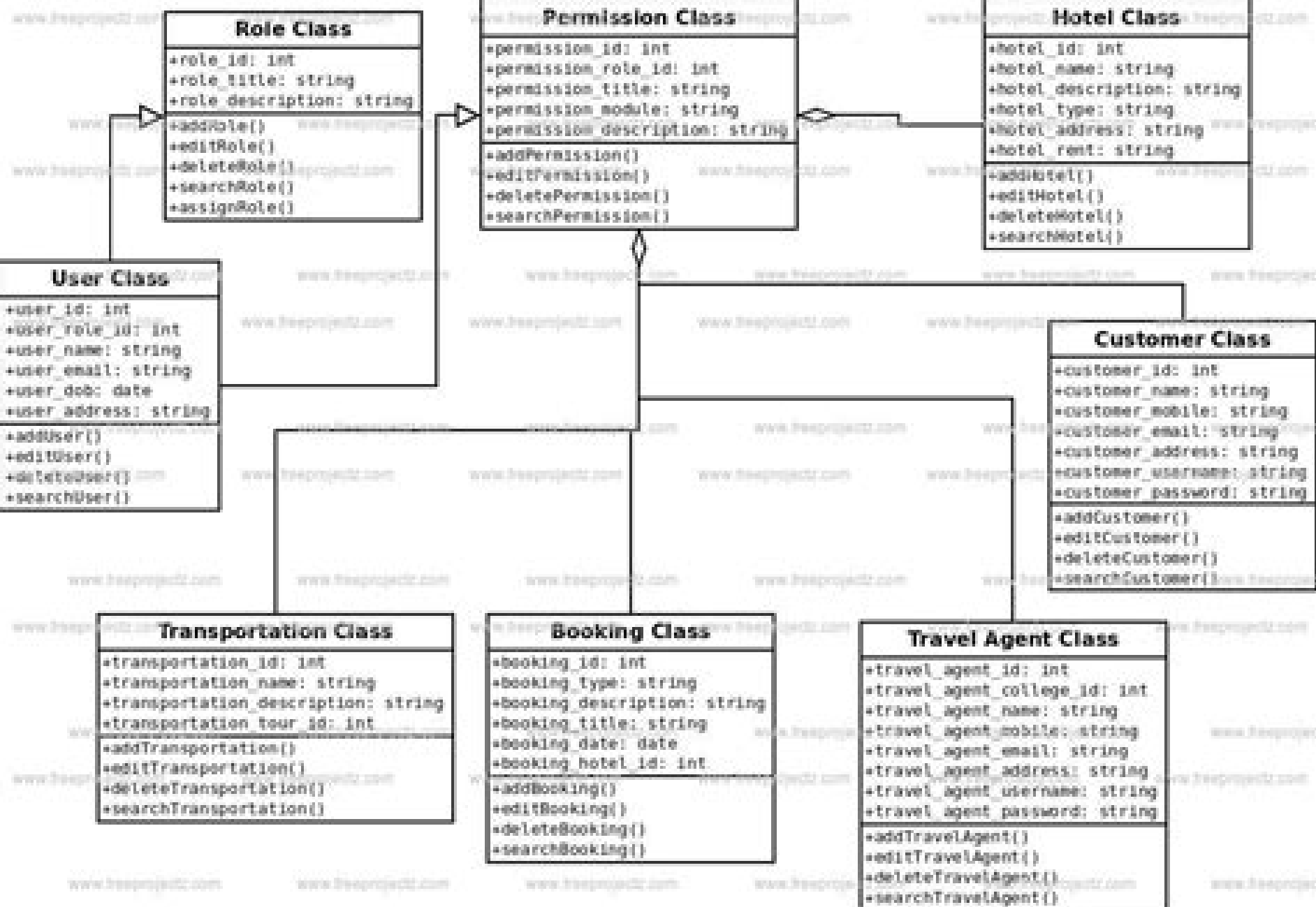
Class Diagram of Tourism Management System
