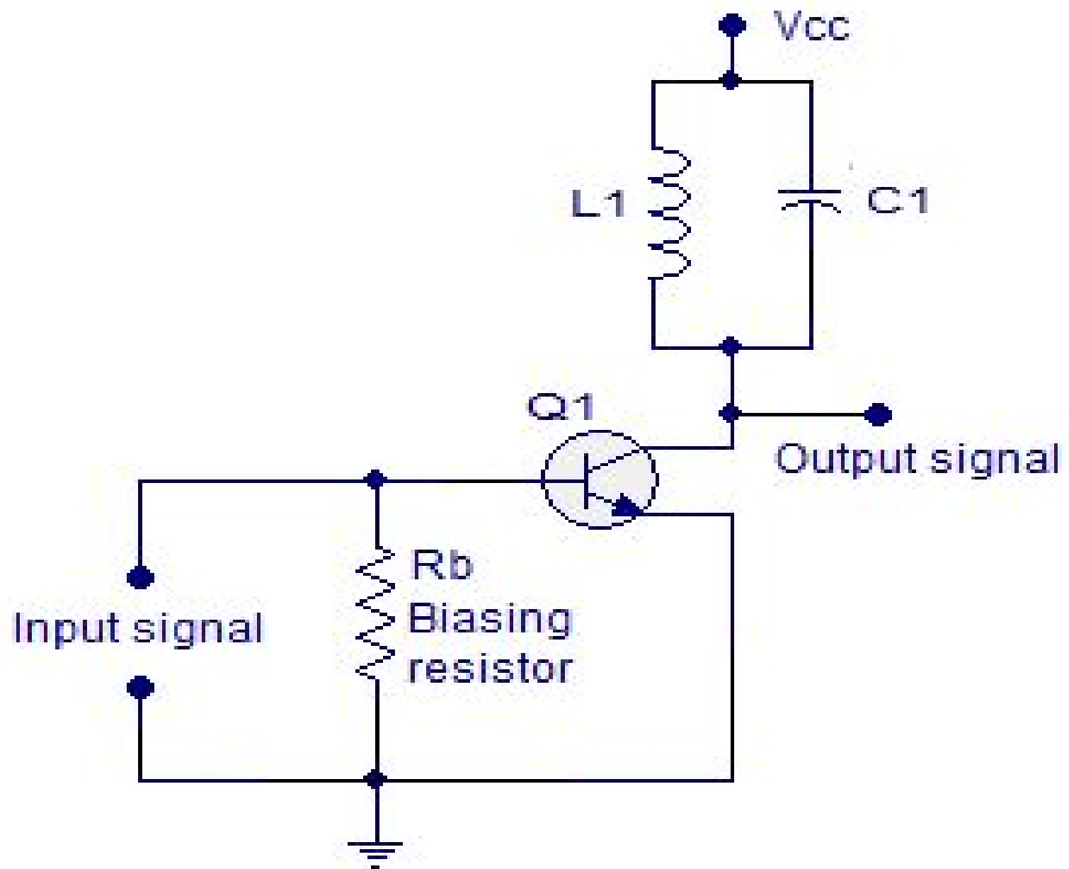
Class C power amplifier
