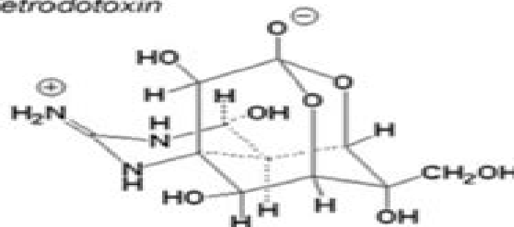
Tetrodotoxin
