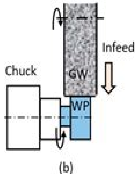
Chuck type cylindrical grinding c=1.0
