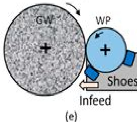
Shoe centerless grinding c=0.5
