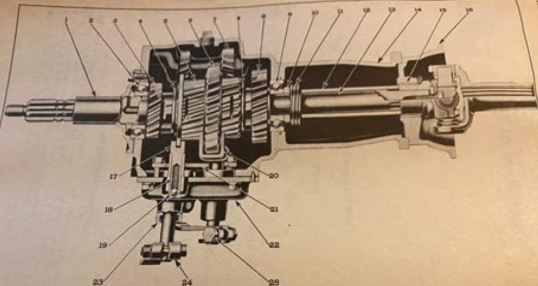
Fig. 1—Transmission Cross Section
