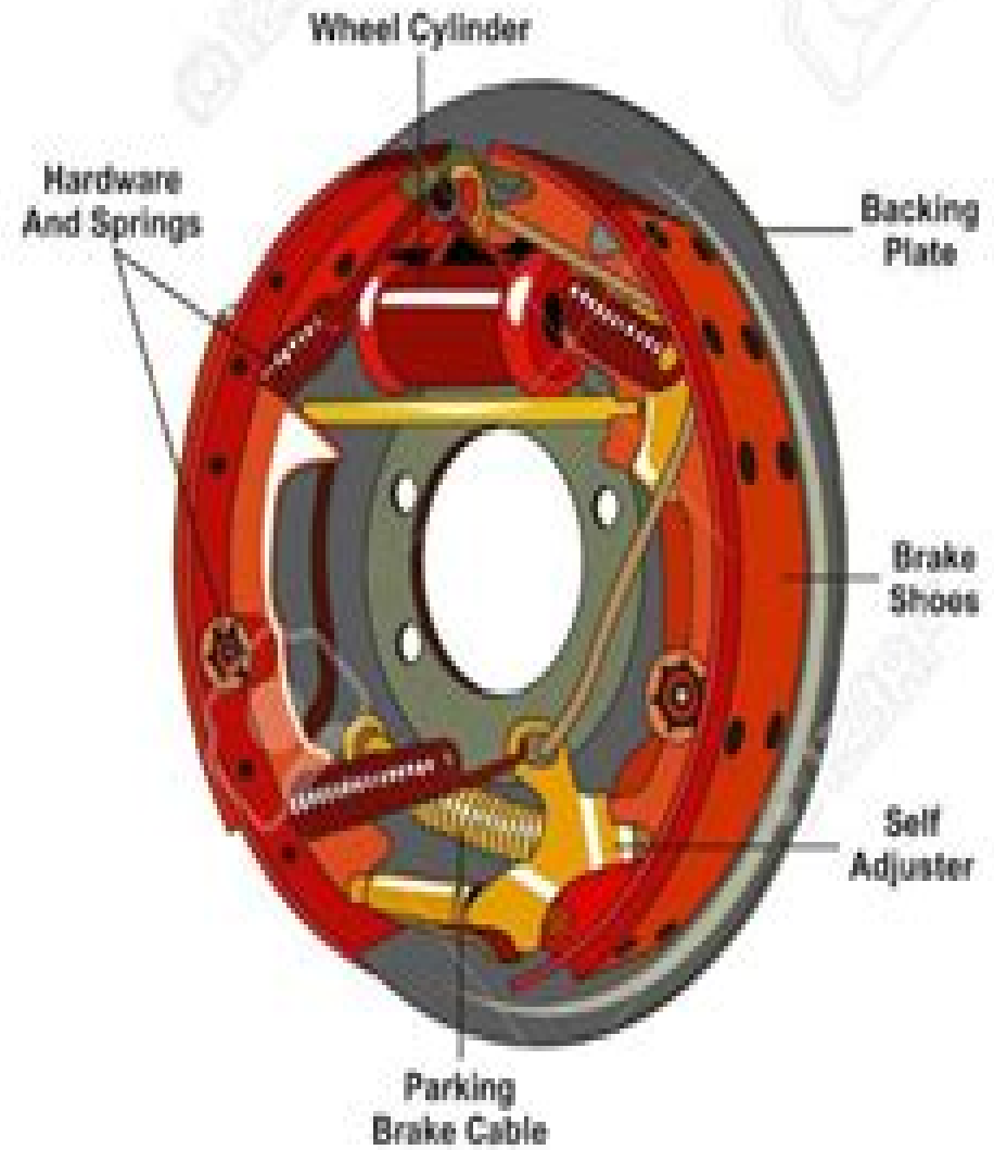
Drum Brake
