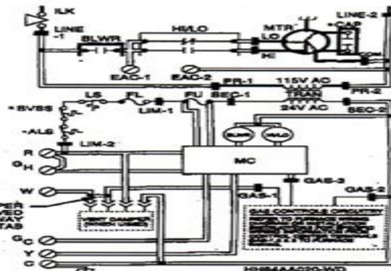
Fig. 2—Wiring Schematic
