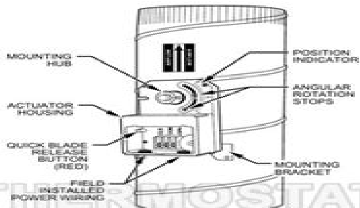
Fig. 1—Damper 24-vac Connections A95096
