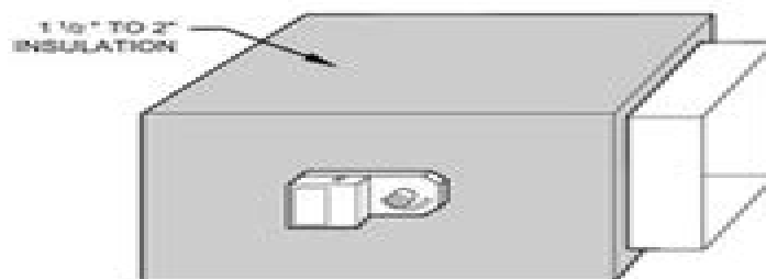
Fig. 4—Insulated Rectangular Metal Duct Work A95134
