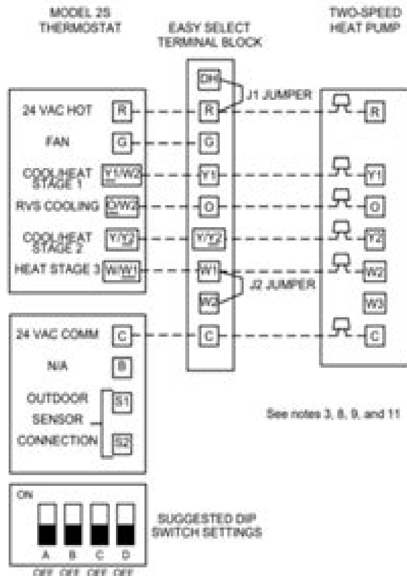
→ Fig. 18—Two-Speed Heat Pump with Variable-Speed Fan Coil (FK, FV, 40FKA)—Model 2S Thermostat
