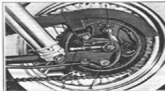
Figure 2B-1A. Adjusting Rear Chain
