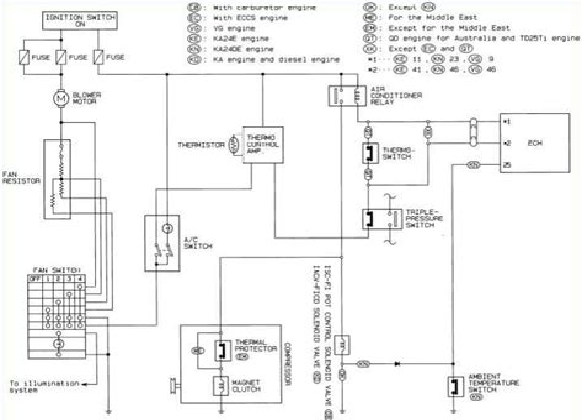
Nissan Navara D22 Air Conditioner Circuit and Wiring System
