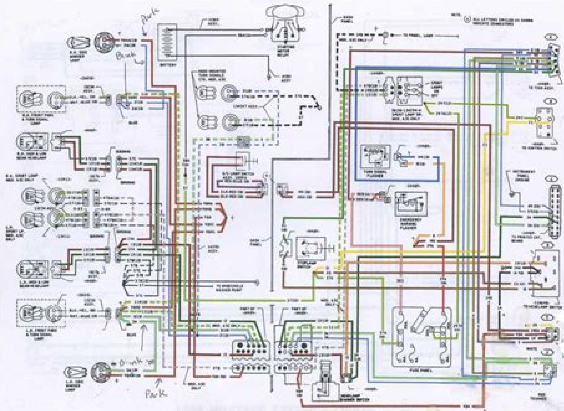
1970 MUSTANG EXTERIOR LIGHTS
