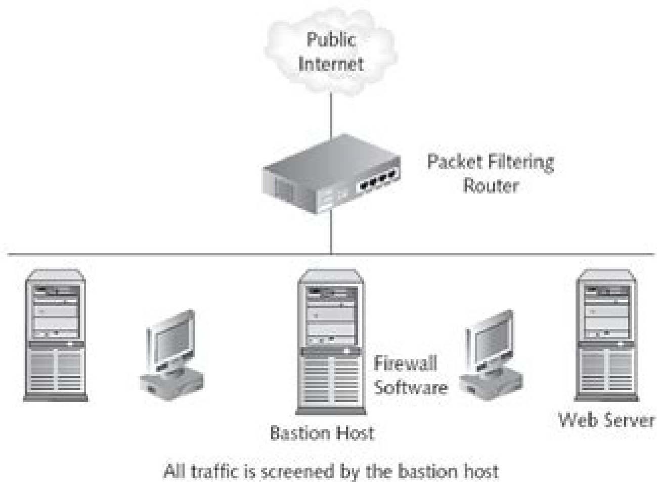
Figure 14-3 Single-homed bastion
