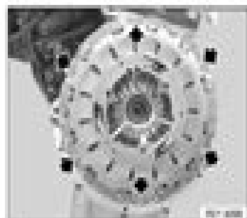
Fig. 19. Mounting S&C Check Bolts On Flywheel Courtesy of BMW OF NORTH AMERICA, INC.
