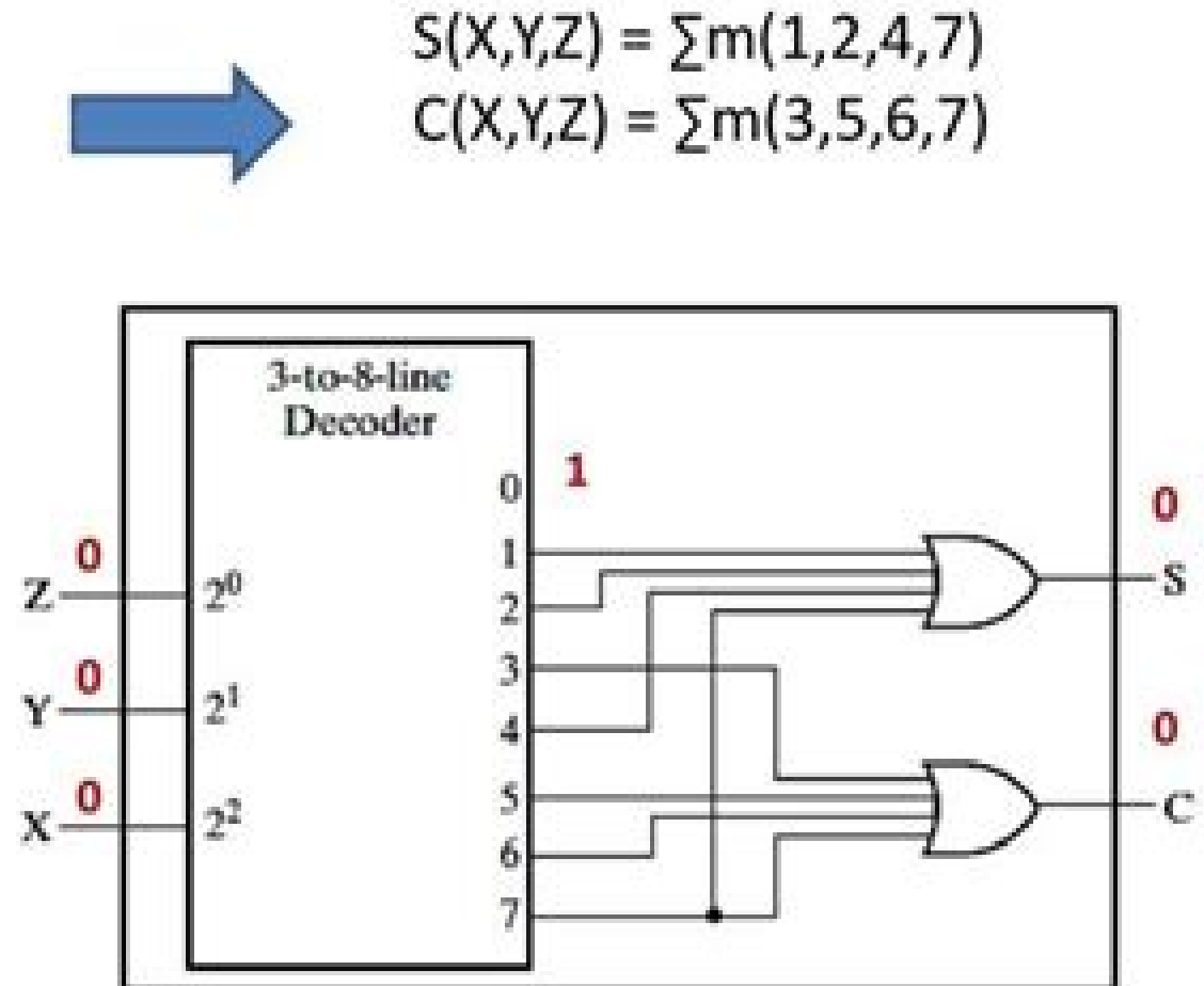
Logic Diagram
