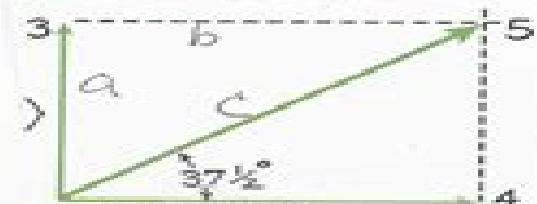
Figure 3.4 \Delta The 3-unit and 4-unit vectors add to produce a resultant vector of 5 units, at 37.5^\circ from the horizontal.
