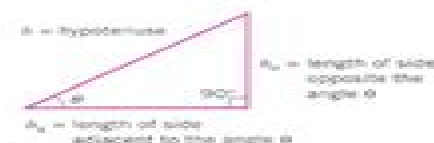
Figure 1.5 A right triangle.
