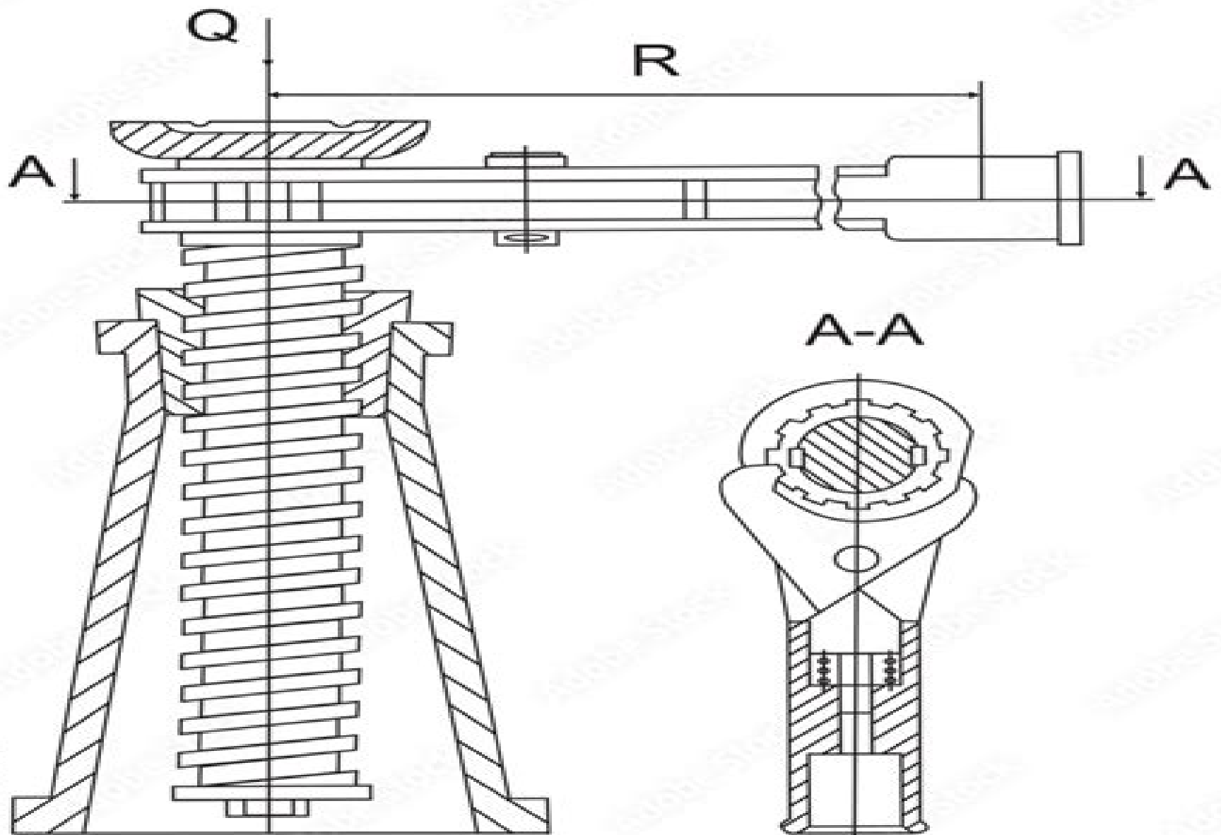
Drawing of the screw jack
