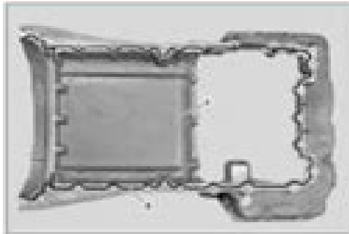
Fig. 31. Identifying Sealant Path For Upper Oil Pan - Engine 3.0L I4 (2007-2009) (Model 14)
