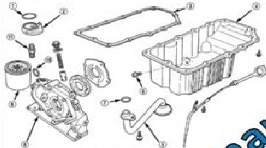
Fig. 114 Oil Pump and Tube
