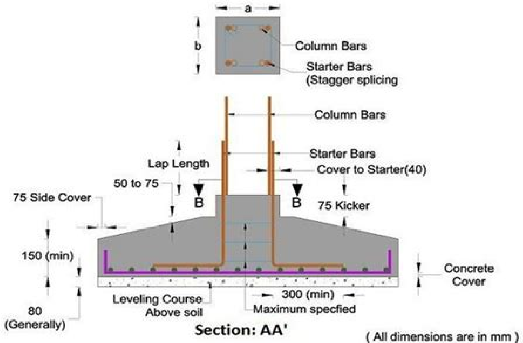
Details of Footing reinforcement
