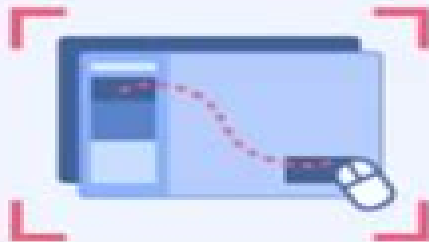
Software Simulation
