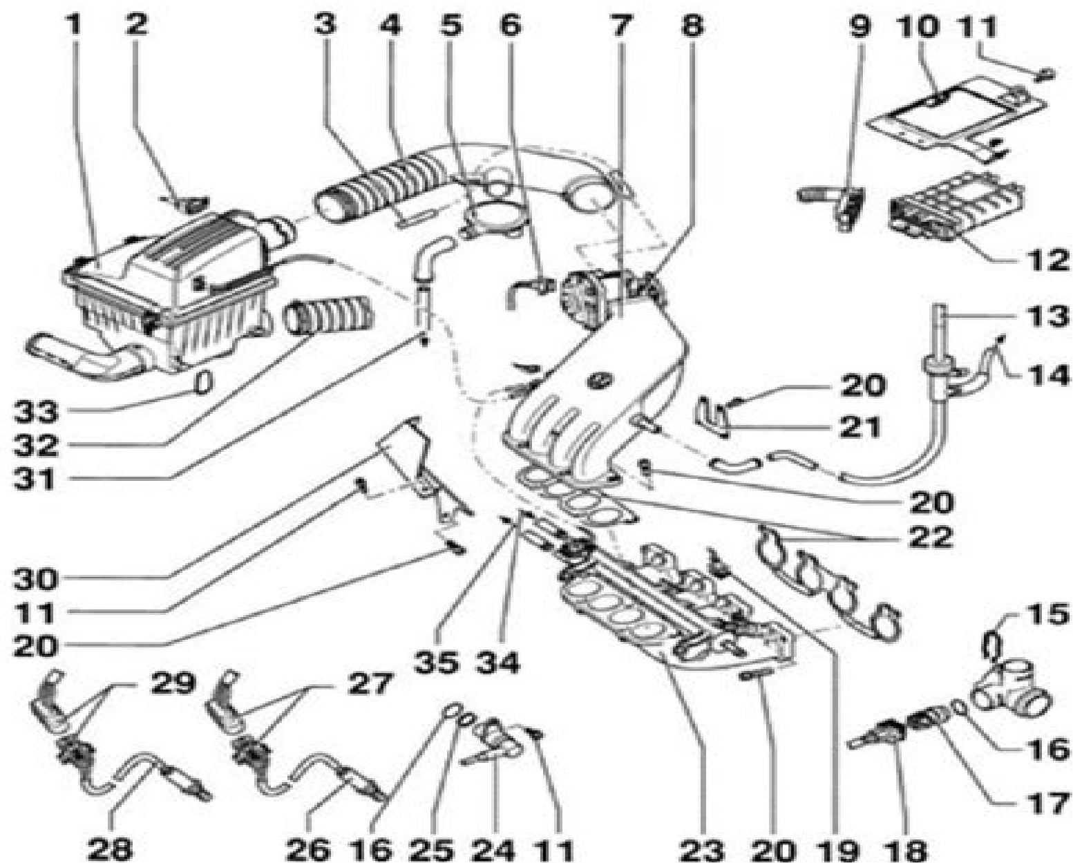
Fig. 2: Identifying Fuel Injection System & Intake Manifold Components Courtesy of VOLKSWAGEN OF AMERICA, INC.
