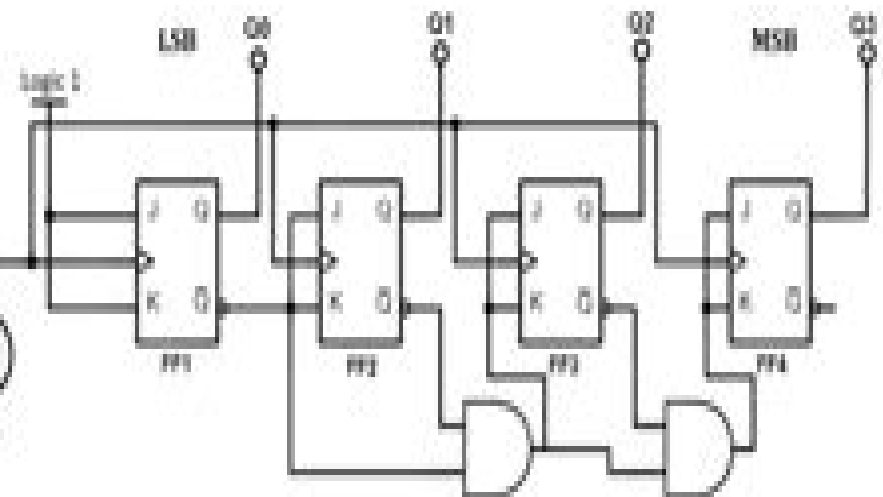
4 Bit Synchronous Down Counter
