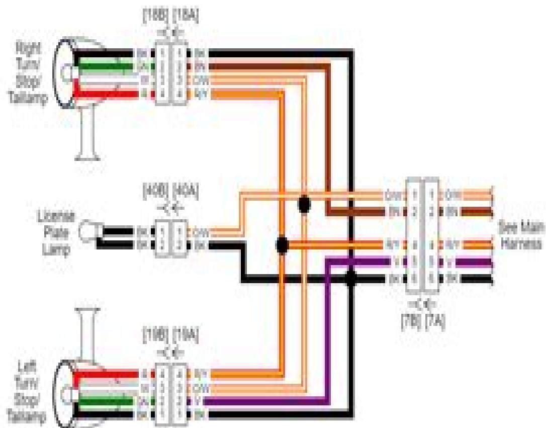
Dual Stop Lamp (Except DCM)
