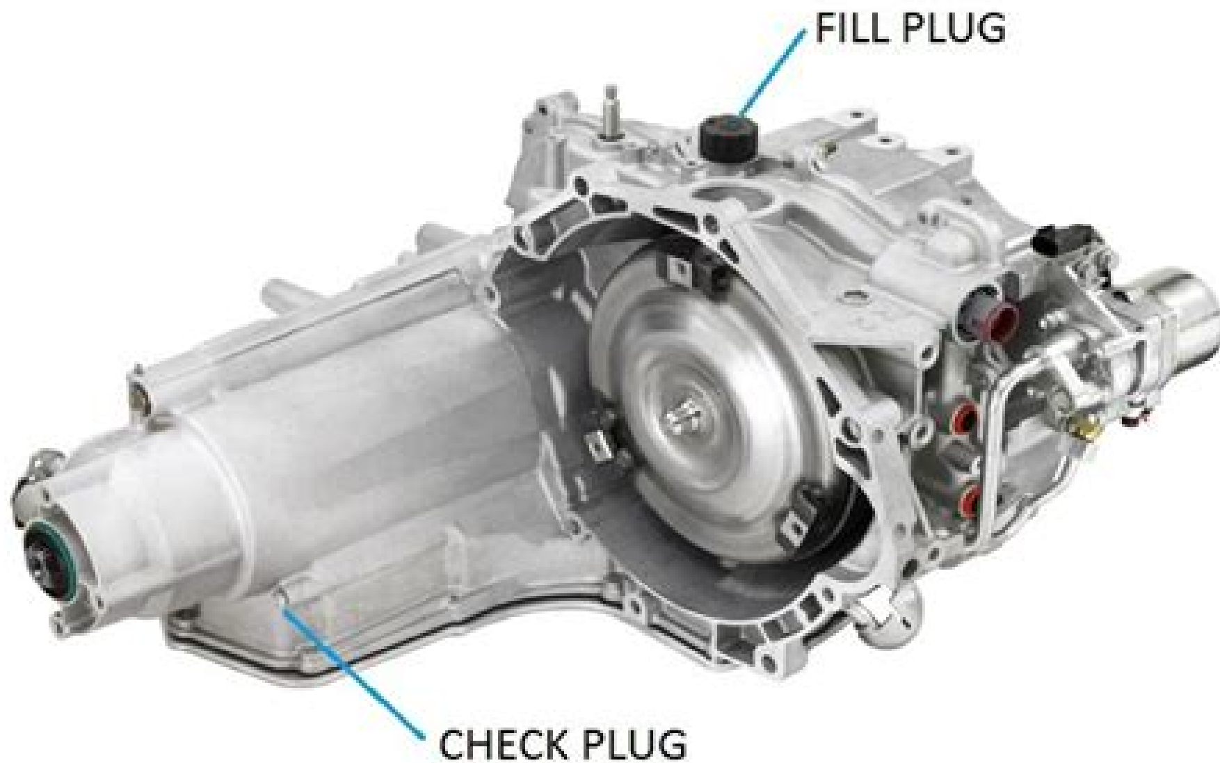
Hydra-Matic 2007 4T45 (4E7) Hybrid Four Speed FWD Automatic Transaxle
