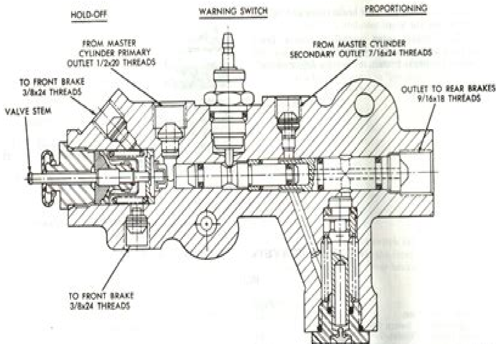
Fig. 1—Combination Warning Switch/Hold-Off/Proportioning Valve Assembly (Sectional View)
