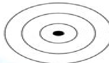
Chlorine (Cl) _____
