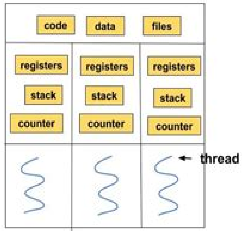
Multi-threaded process
