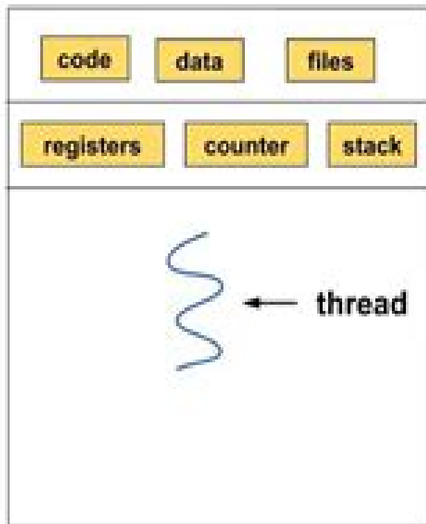
Single-threaded process
