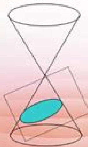
ELLIPSE
