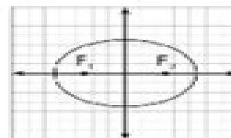
Ellipse
