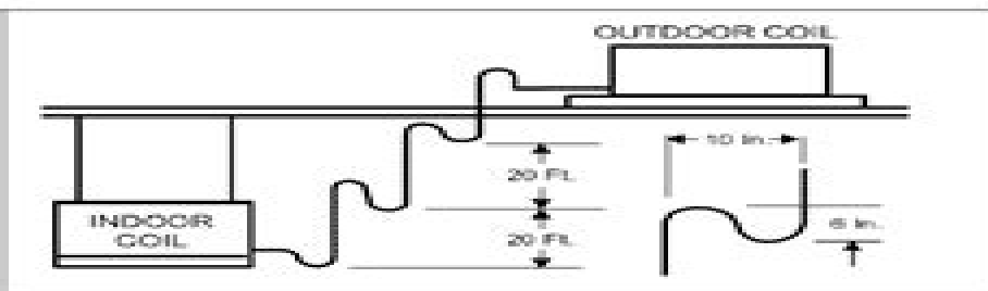
FIGURE 2: Oil Trap
