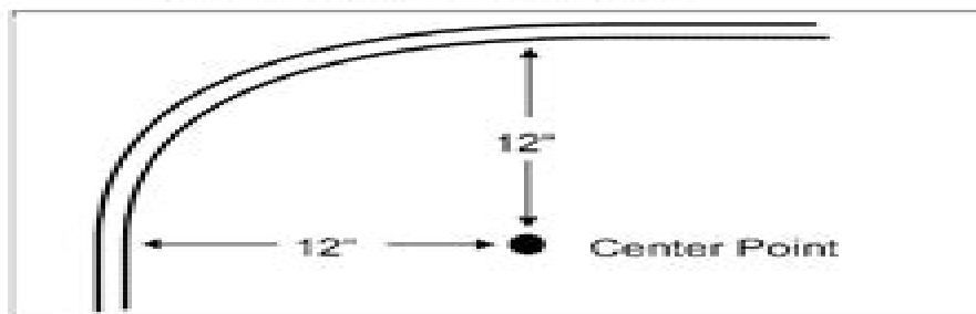
FIGURE 3: Minimum Suction Line Form
