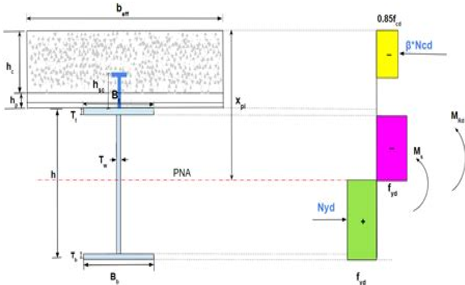
CROSS-SECTION OF COMPOSITE BEAM
