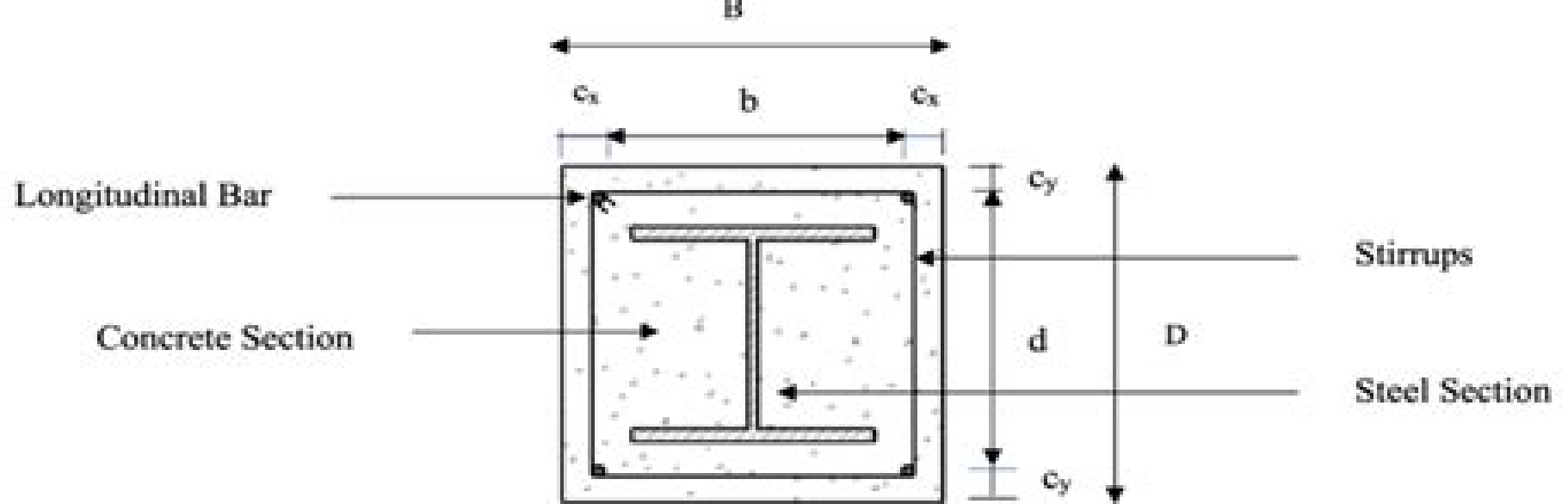
(a) Sectional View of Composite Column Section
