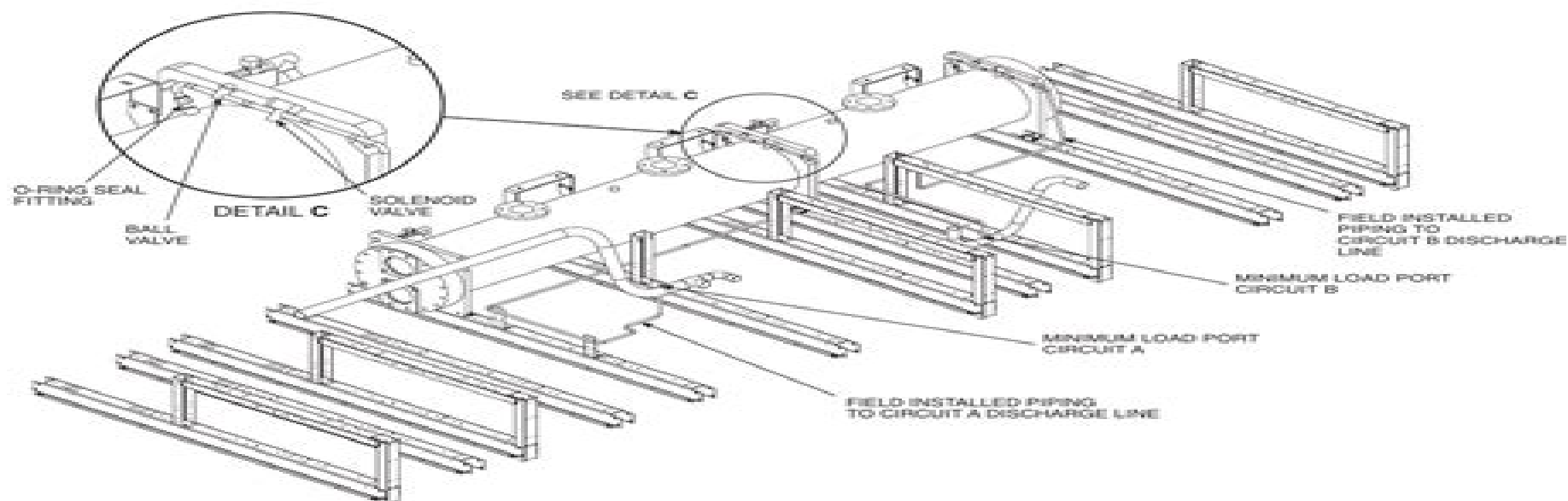
Fig. 3B — Typical Piping and Valve Installation 30GXN,R204-350 and Associated Modular Sizes (204-268 Shown)
