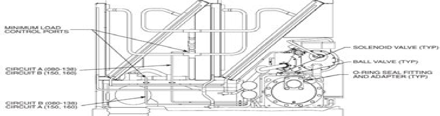
Fig. 3A — Typical Piping and Valve Installation 30GXN,R080-178 and Associated Modular Sizes (080-150, 160 Shown)
