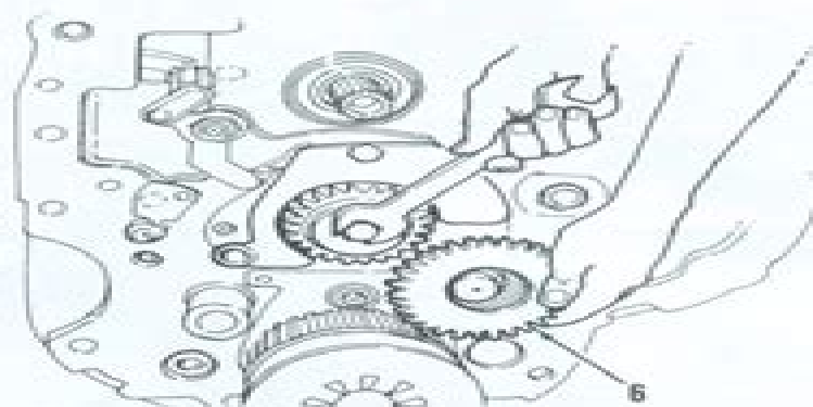
Fig. 16—Rotate drive pinion shaft until idler gear (6—Fig. 15) can be removed. Idler gear can be removed in only one position.
