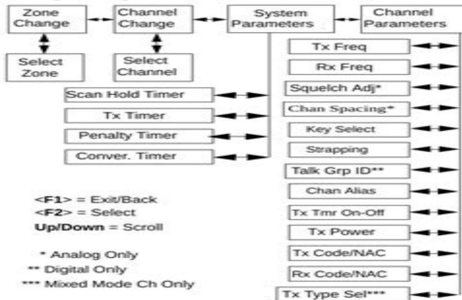
Figure 5.1 Keypad Programming Menu Flowchart
