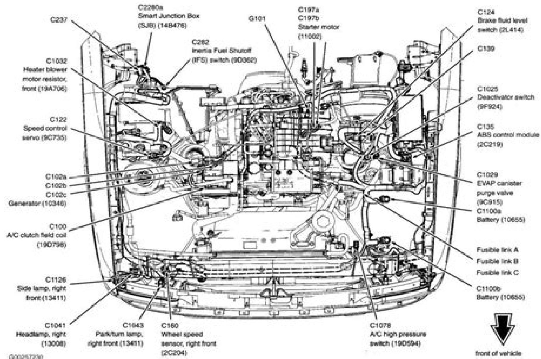
Fig. 1: Engine Compartment
