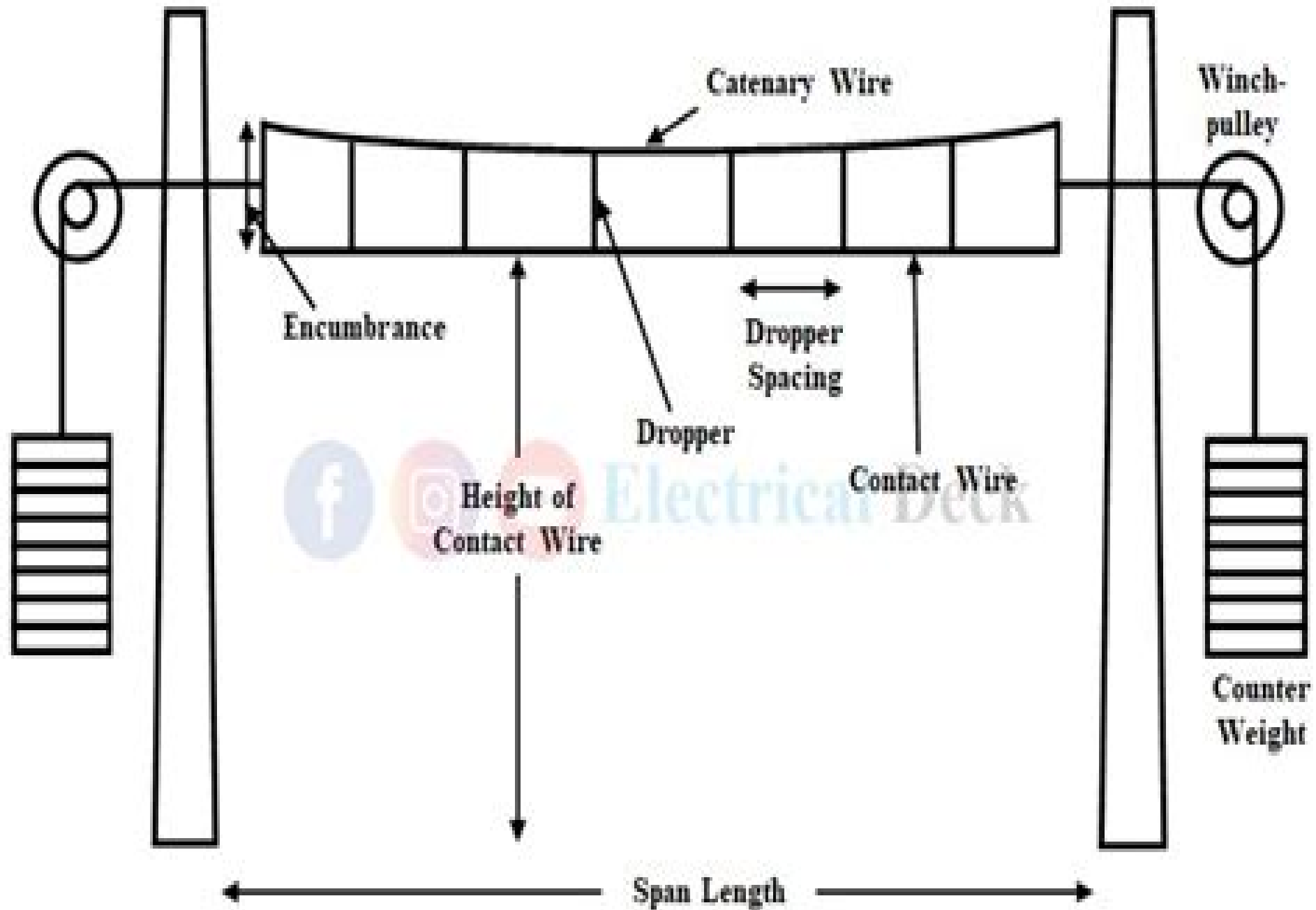
Design of Overhead Equipment in Traction System
