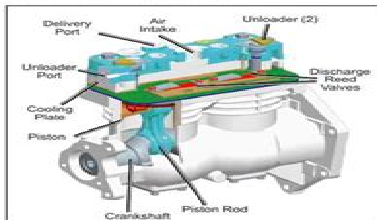
FIGURE 2 - BA-922® COMPRESSOR (CUT-AWAY)
