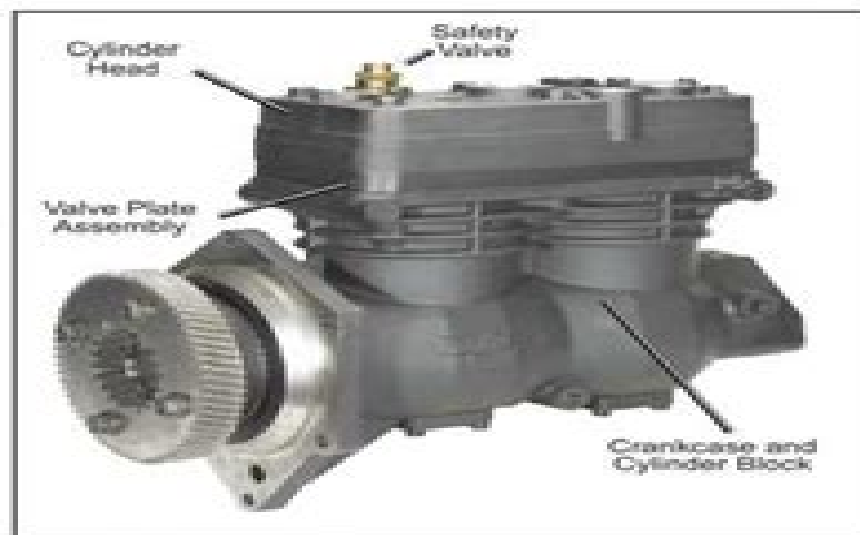
FIGURE 1 - BA-922® COMPRESSOR
